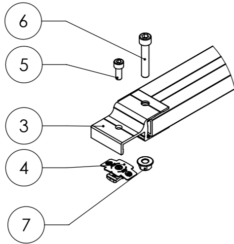
Detail Z 1:5
